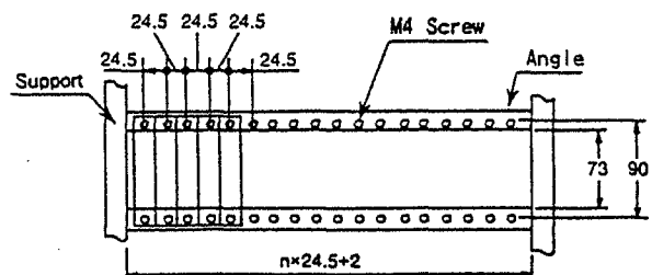
Fig.5 Angle Mounting Dimensions
