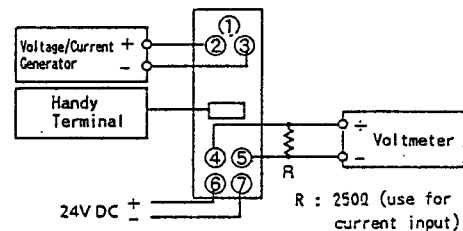
Fig.11 Connection to Handy Terminal
