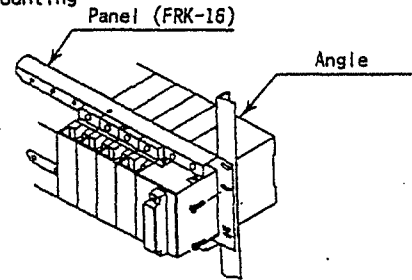
Fig.1 Rack Mounting
