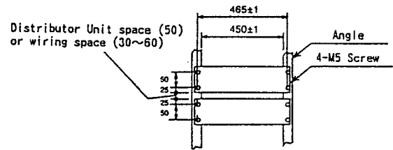
Fig.7 Panel Mounting Dimensions
