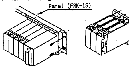
Fig.2 Wall Mounting
